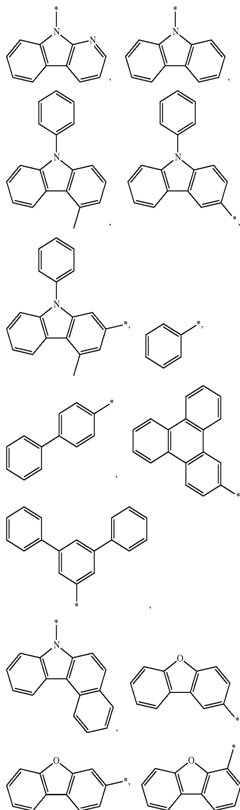
[Group II-1]
