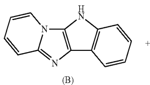
[Reaction Scheme 6]
