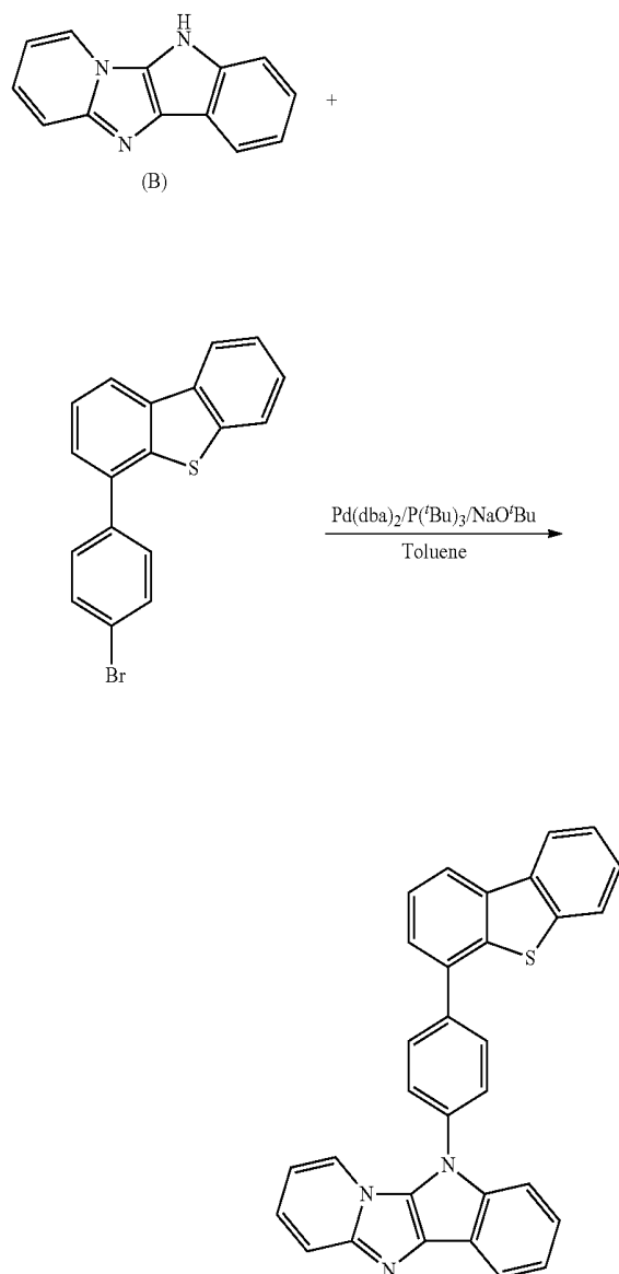
[Reaction Scheme 11]
