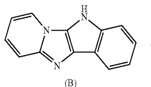
[Reaction Scheme 10]
