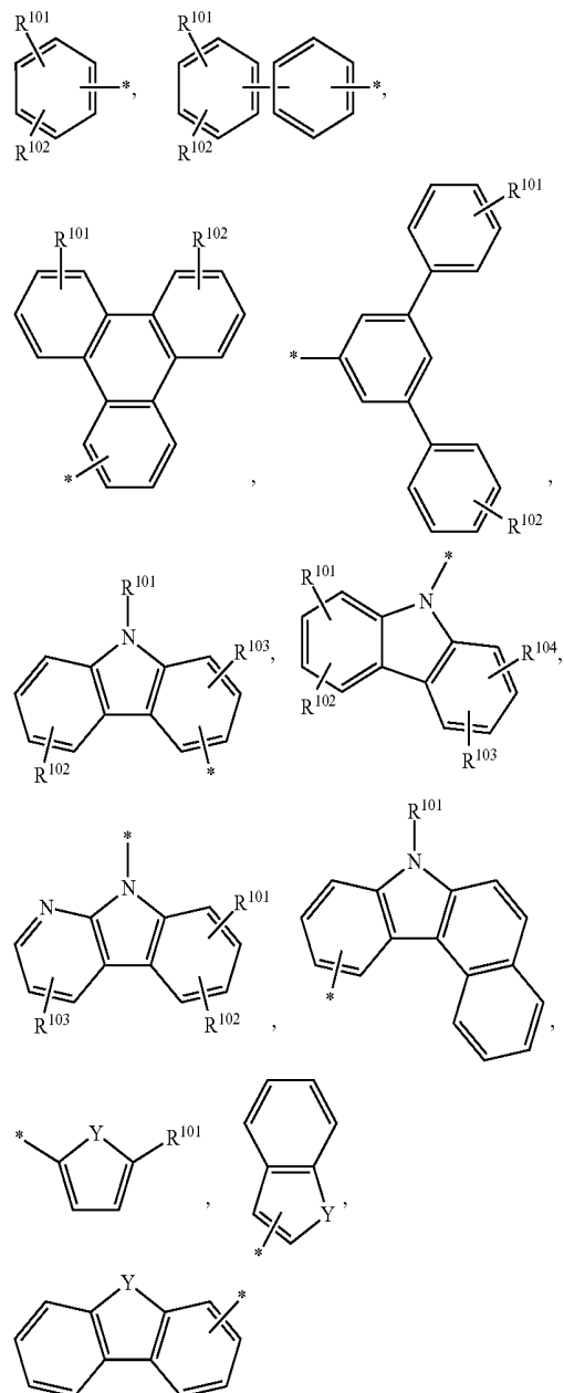
[Group II]
