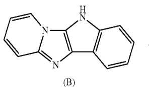
[Reaction Scheme 7]
