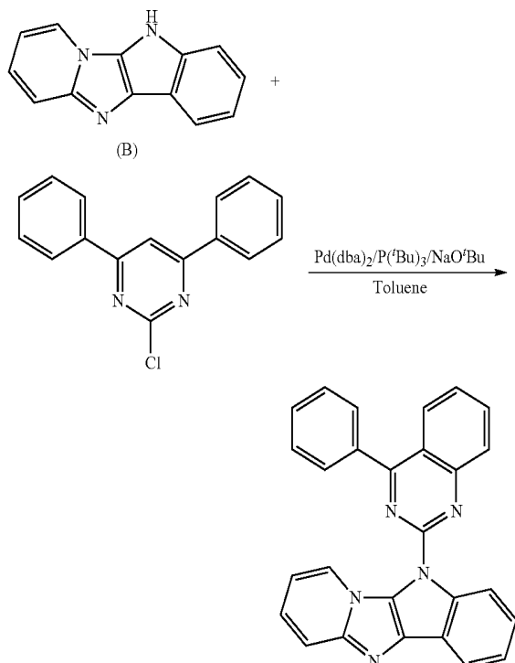
[Reaction Scheme 5]
